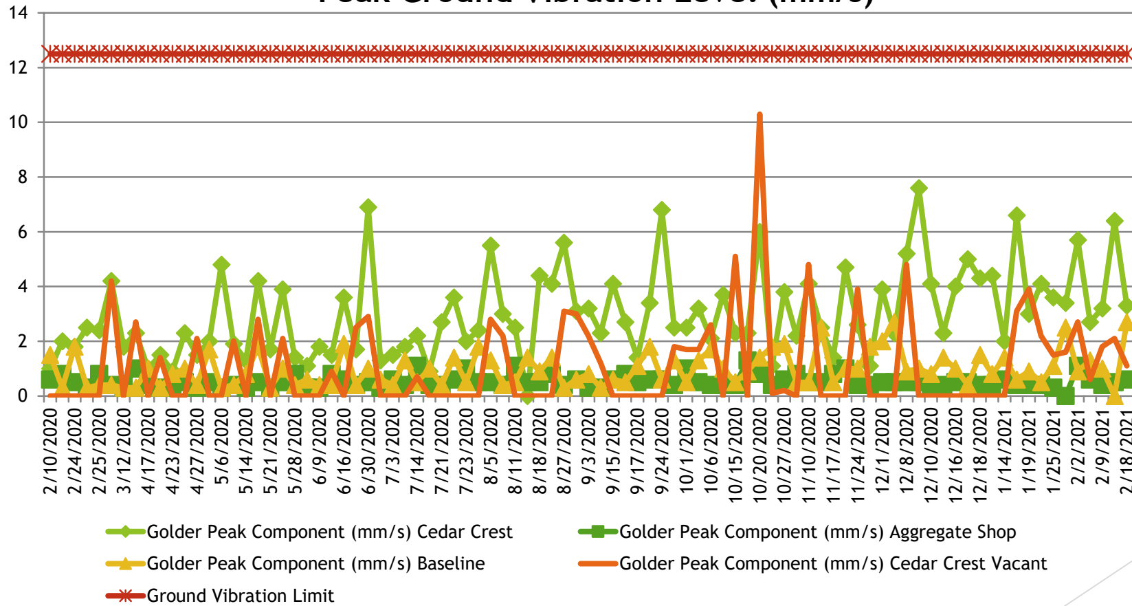
Peak Ground Vibration Level (mm/s)
