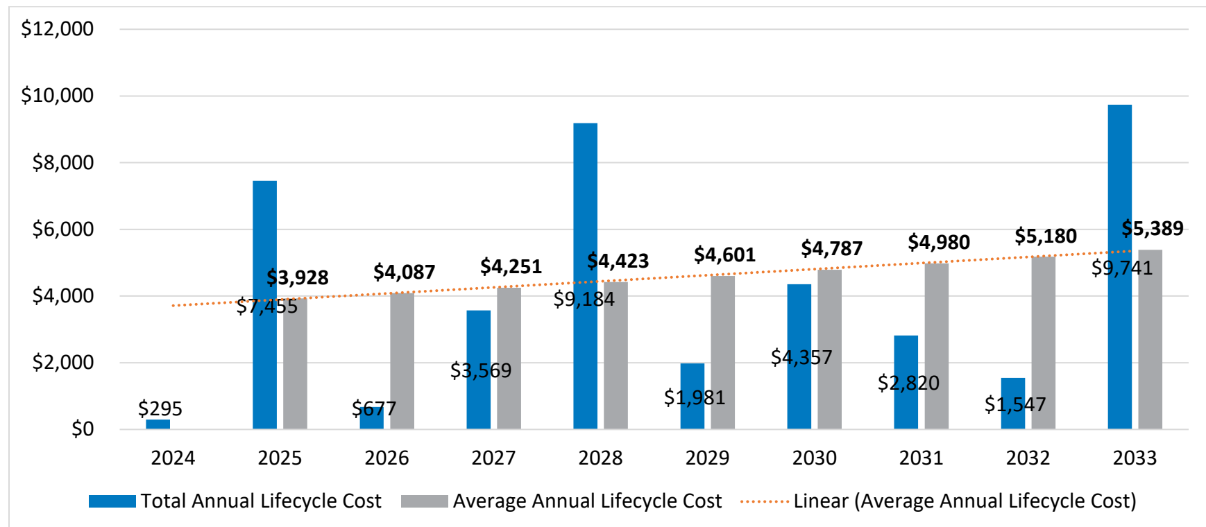
Figure G6 - Total Annual Lifecycle Cost vs Average Annual Lifecycle Cost ($,000's) – Reduce Backlog
